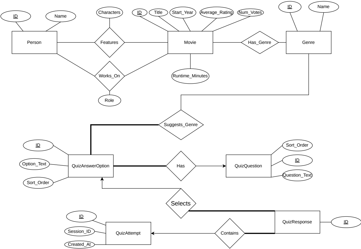
Movie Match E/R diagram
